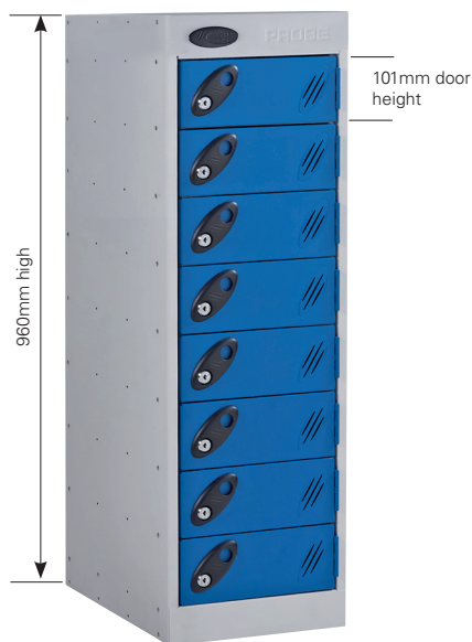
8 compartment multi-door
